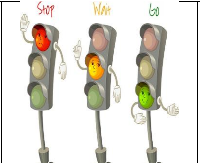
traffic lights
