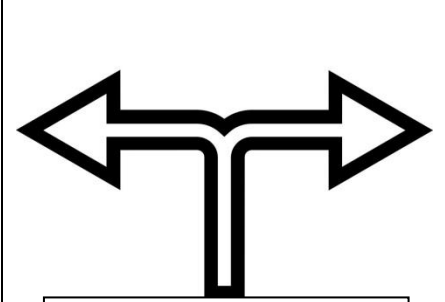
T-junction
