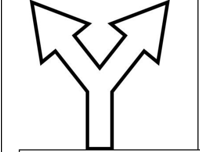
Y-junction
